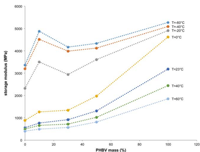
Figure 10. Isothermal E' values [at various temperatures ( T_s )] as a function of the blend composition. [Color figure can be viewed in the online issue, which is available at wileyonlinelibrary.com .]
